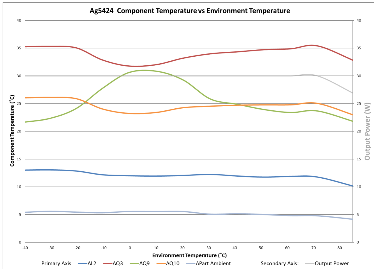
Ag5424 delta component temperature
