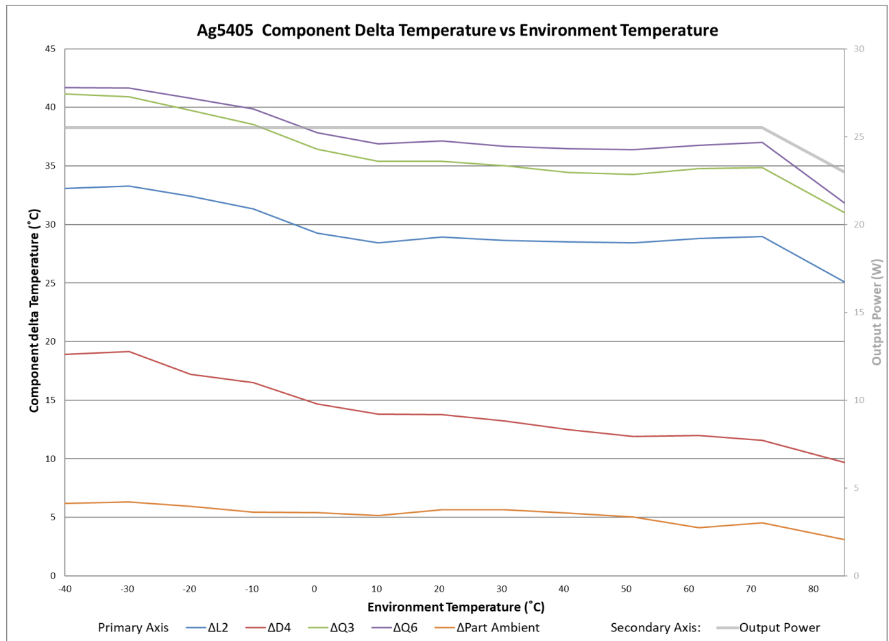
Ag5405 delta component temperature
