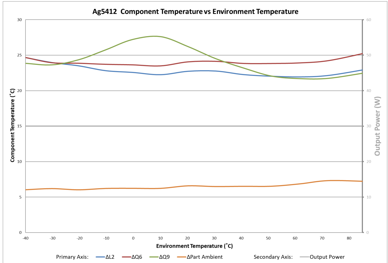
Ag5412 delta component temperature
