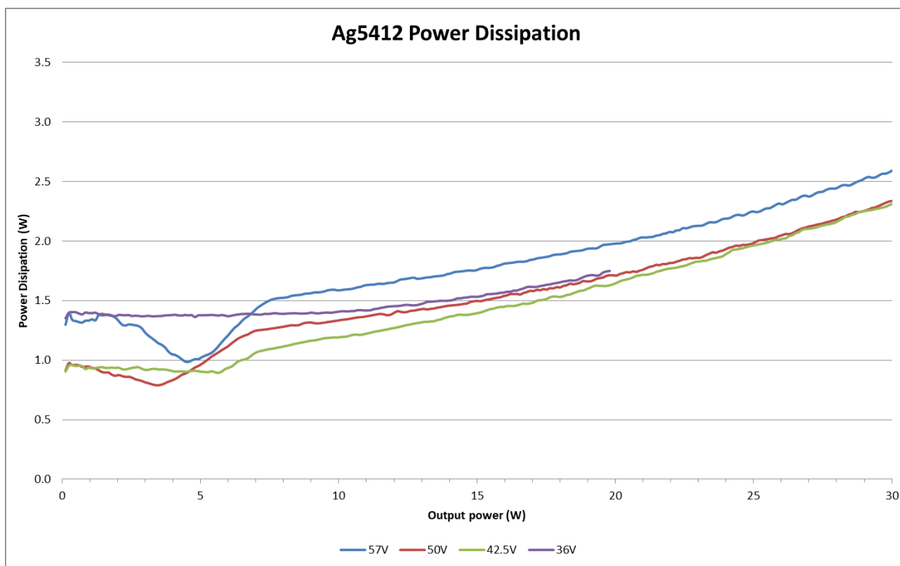
Ag5412 power dissipation vs load
