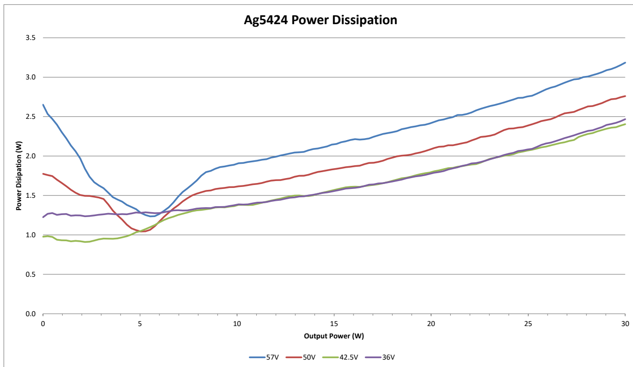
Ag5424 power dissipation vs load
