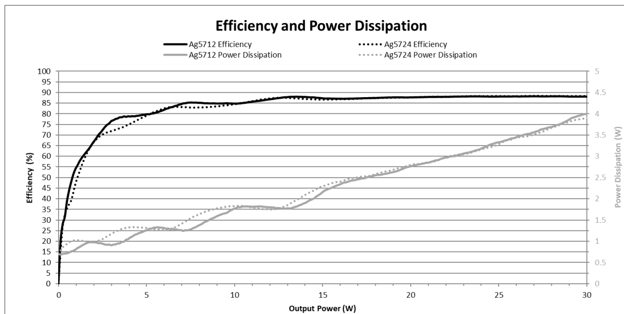
Figure 7: Ag5700-LPB Efficiency
