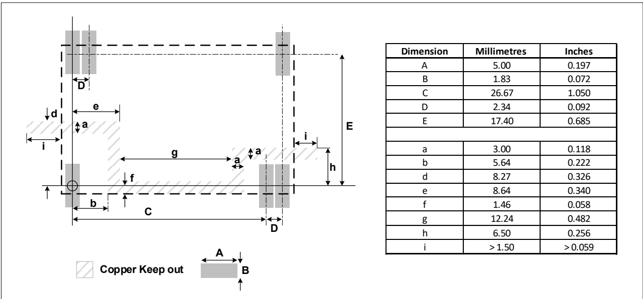
Figure 15: Land Pattern
