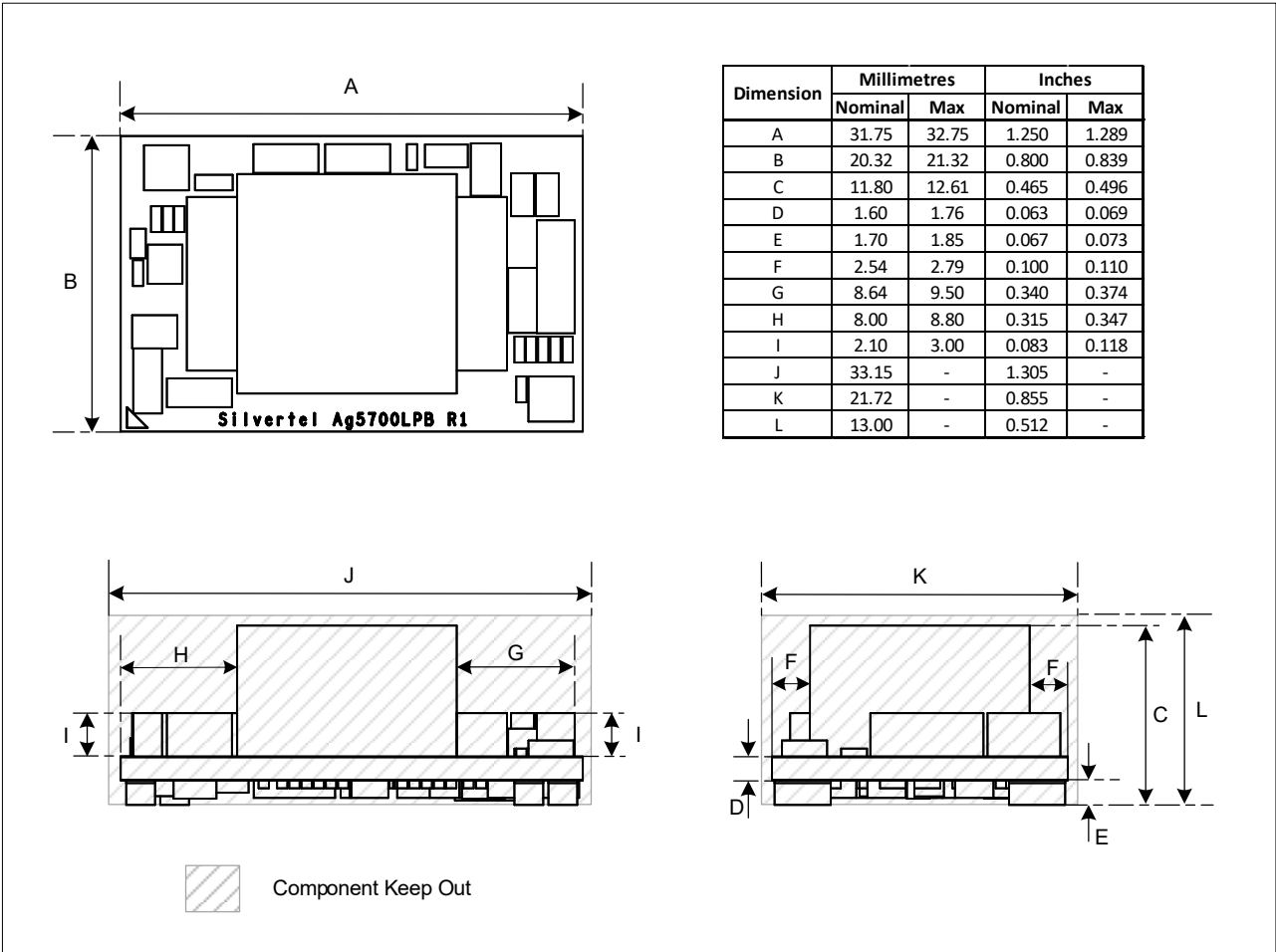
Figure 14: Package Dimensions
