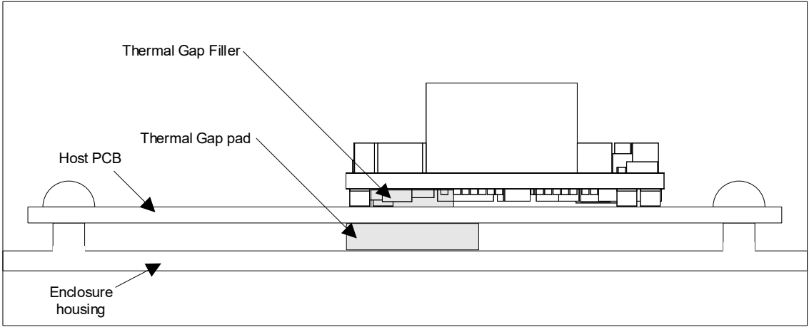
Figure 11: Additional Heatsinking
