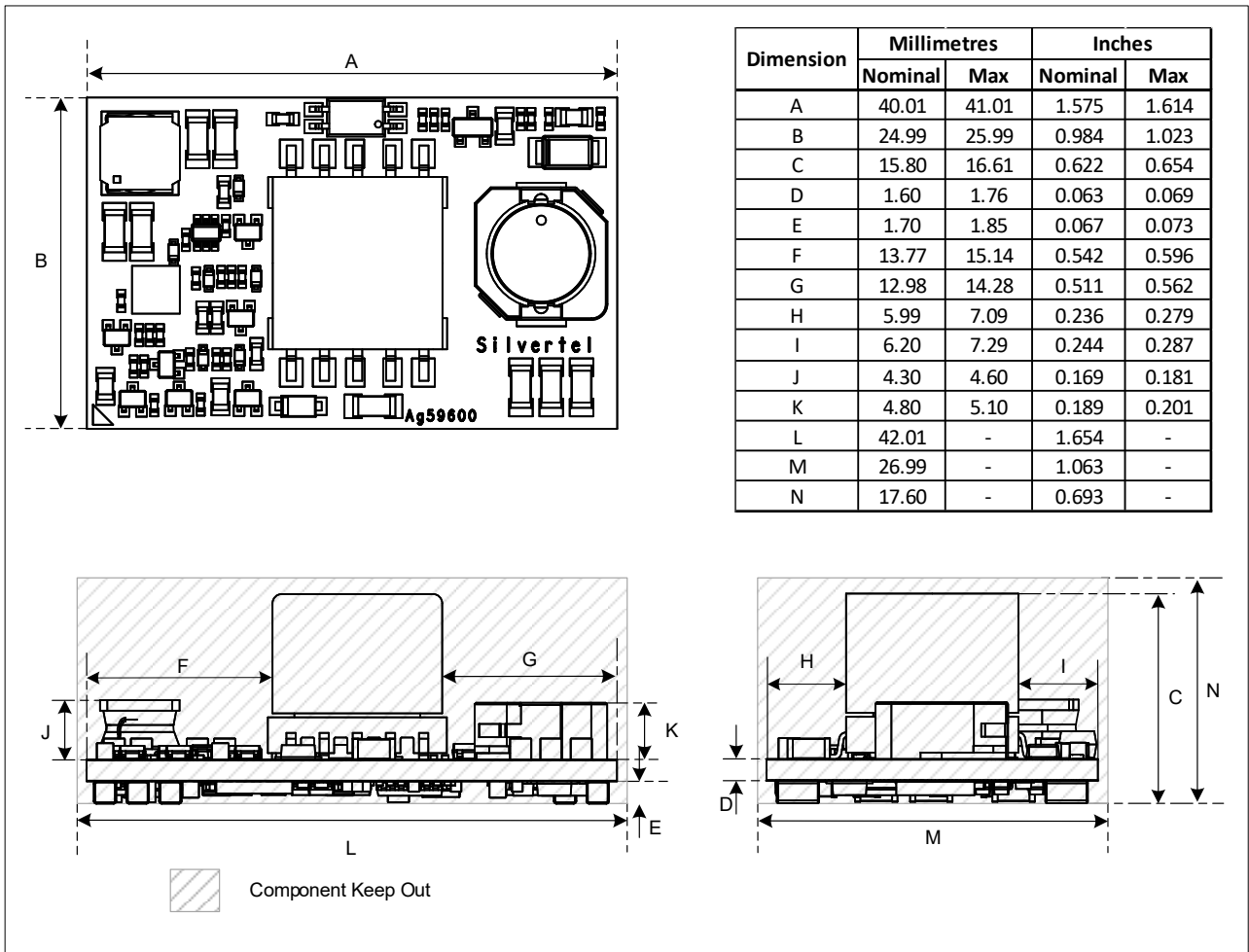
Figure 12: Package Dimensions
