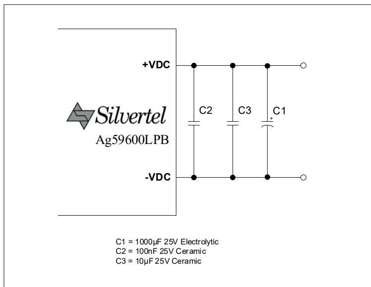
Figure 6: Output Filter
