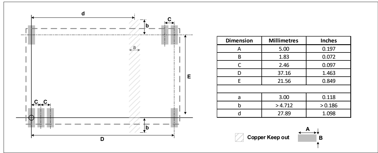
Figure 13: Land Pattern
