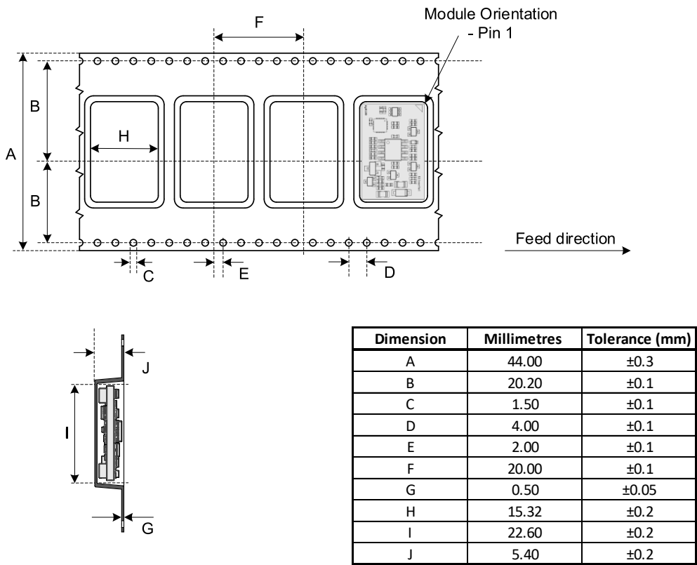
Figure 16: Tape Dimensions
