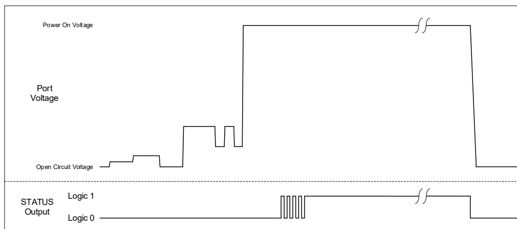
Figure 11: STATUS Output at Port Connect and Disconnect
