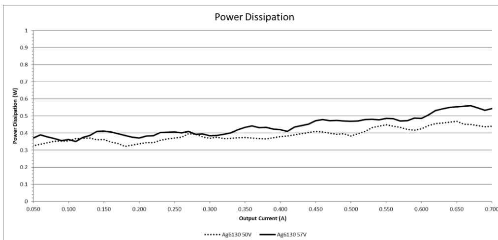
Figure 8: Power Dissipation vs Output Current
