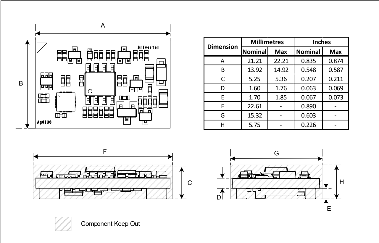
Figure 13: Package Dimensions
