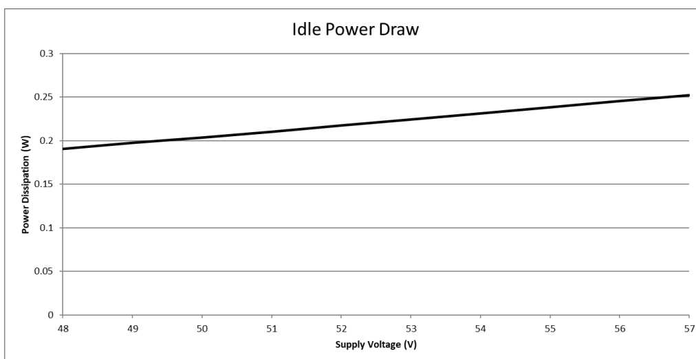
Figure 9: Idle Power Draw
