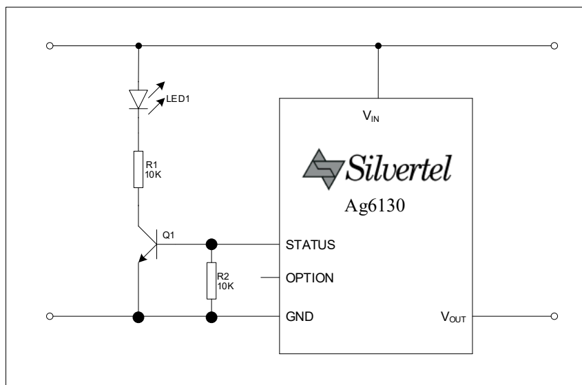
Figure 10: STATUS Output Configuration
