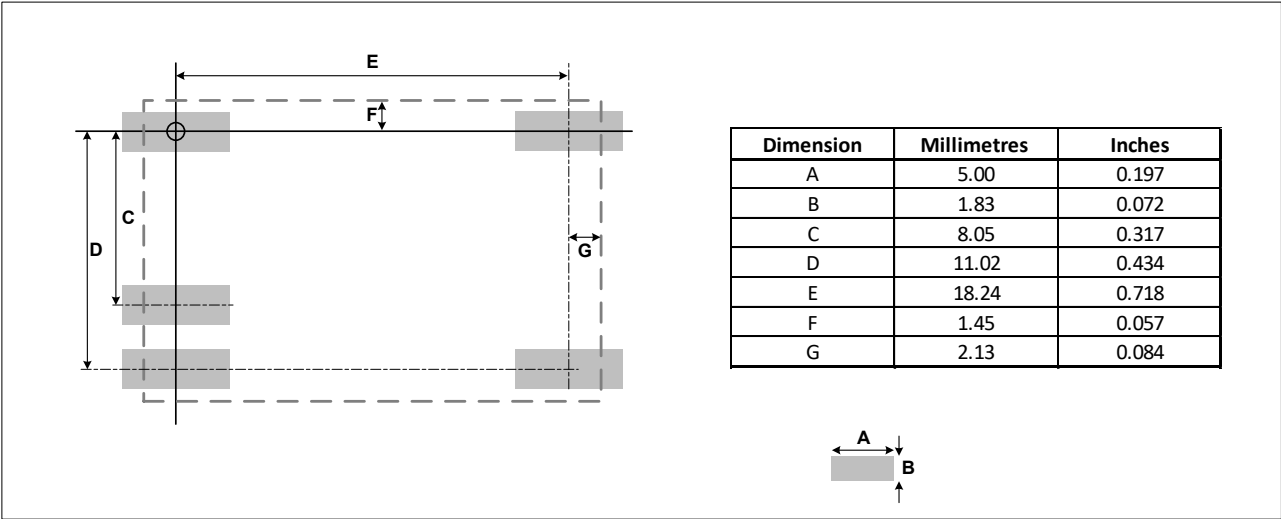
Figure 14: Land Pattern
