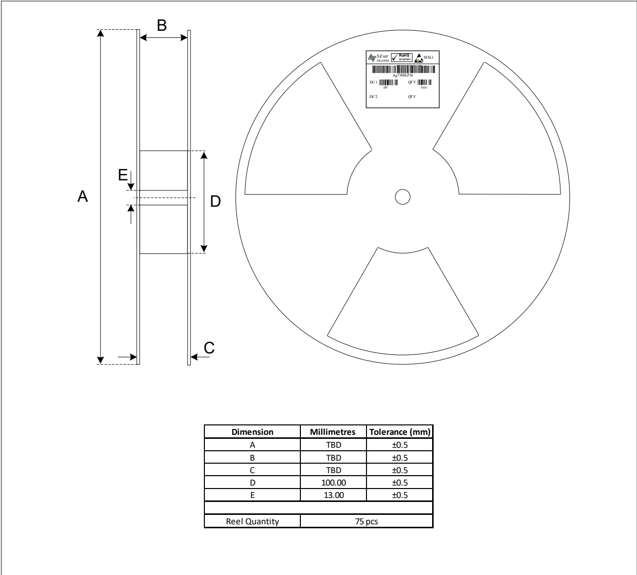
Figure 16: Reel Dimensions
