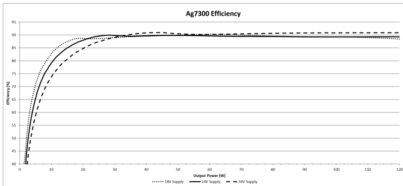
Figure 6: Ag7300 Efficiency
