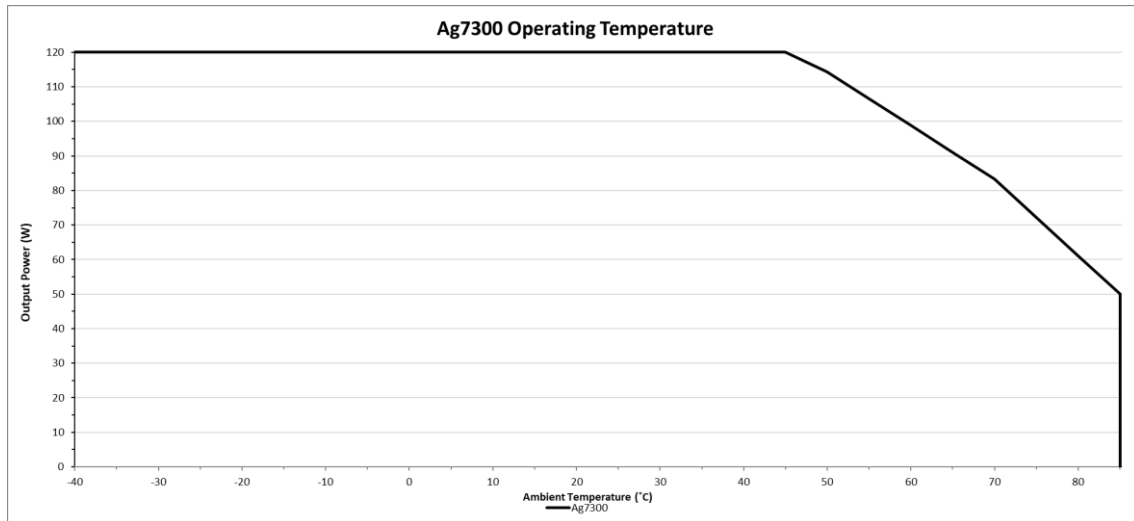
Ag7300 operating temperature profile
